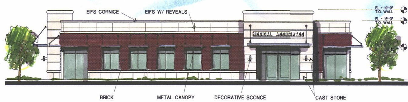
02 FRONT ELEVATION 1/16"=1'-0" SCHEME 1
