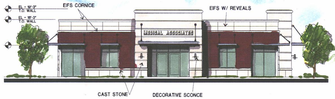
01 SIDE ELEVATION 1/16"=1'-0" SCHEME 1
